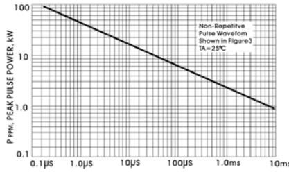
FIGURE 1-PEAK PULSE POWER VS PULSE TIME
