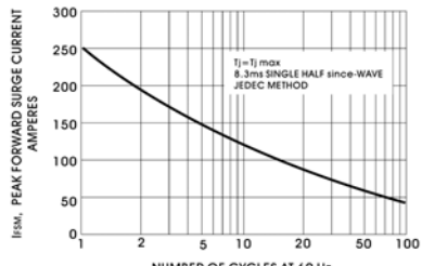
FIG. 6-MAXIMUM NON-REPETITIVE PEAK FORWARD SURGE CURRENT UNIDIRECTIONAL
